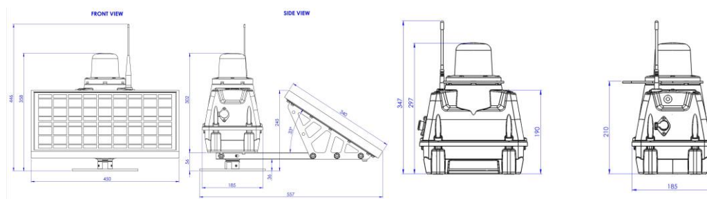
Figure 1.3. Technical drawings of SP-401 Solar and Portable Airfield Lights
